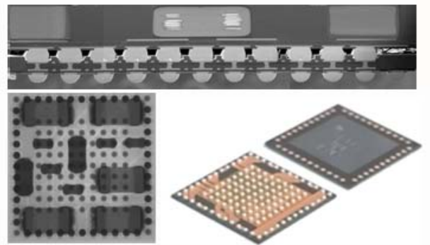
Figure 9. Photographs of 3D SiP eWLB-PoP with discretes on interposer or top package of discretes.
