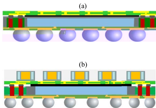
Figure 7. Schematics of 3D eWLB SiP: (a) with interposer and (b) discretes on interposer or top package of discretes.
